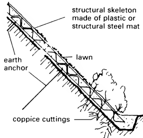
10 Preserving bank surface with structural skeleton
